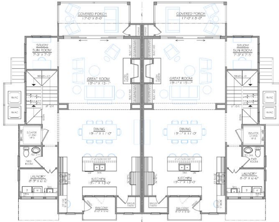
FIRST FLOOR 10' CEILING HEATED SQ FT: 1101 UNHEATED SQ FT: BALCONY 42 REAR PORCH 144
