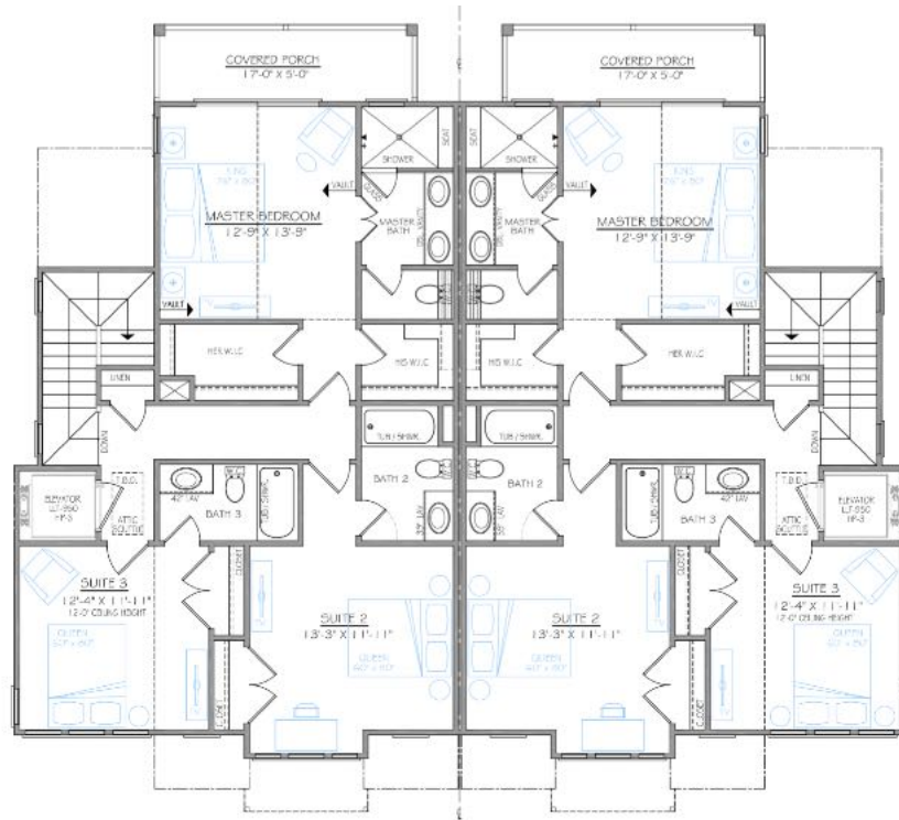
SECOND FLOOR 9' CEILING, 12' VAULTED CEILING, MASTER BEDROOM HEATED SQ FT: 1001 UNHEATED SQ FT: REAR PORCH 85
